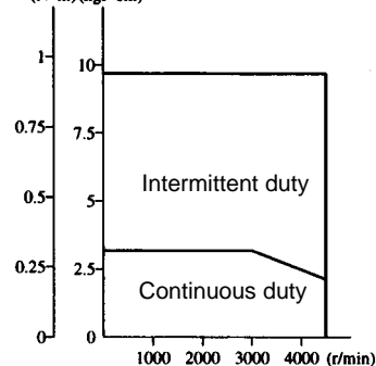
R88M-U75030HA (N·m)(kgf·cm)
