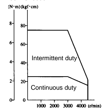
R88M-U75030HA (N·m)(kgf·cm)
