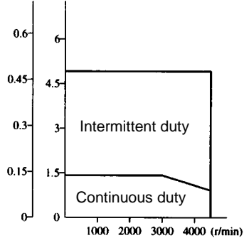
R88M-U30030LA (N·m)(kgf·cm)
