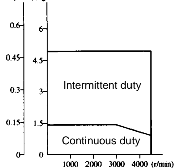
R88M-U40030HA (N·m)(kgf·cm)
