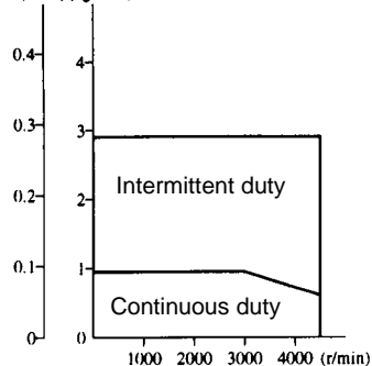
R88M-U20030HA (N·m)(kgf·cm)
