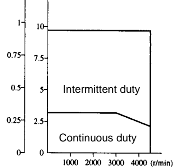
R88M-U10030LA (N·m)(kgf·cm)
