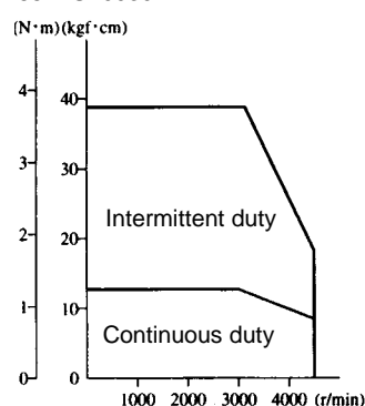
R88M-U40030HA (N·m)(kgf·cm)
