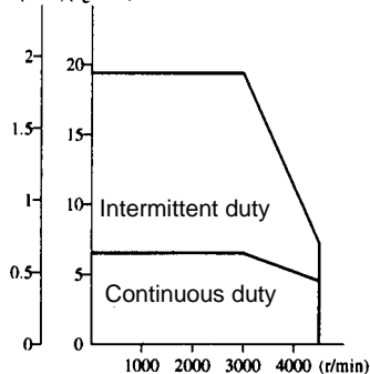
R88M-U20030LA (N·m)(kgf·cm)
