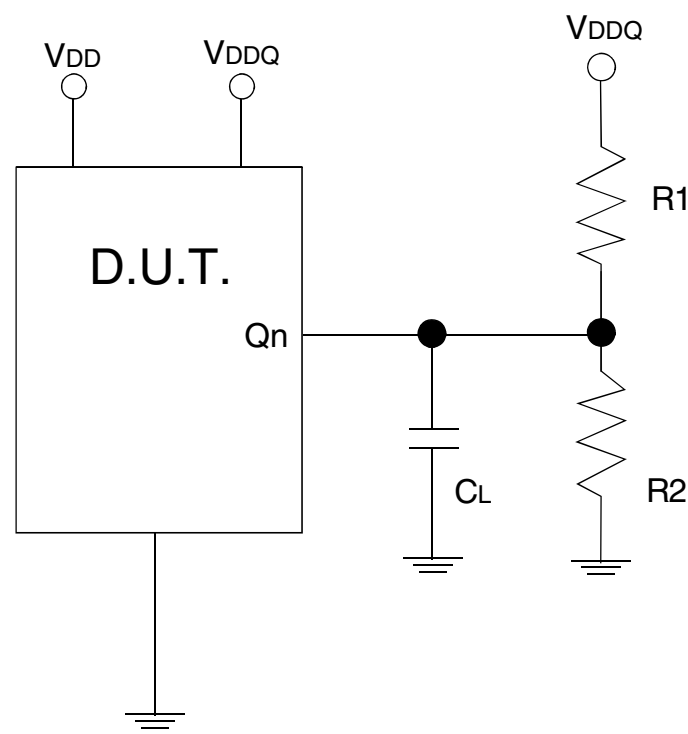
Test Circuit for SDR Outputs
