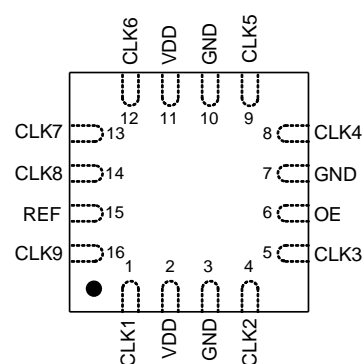
QFN-16L
