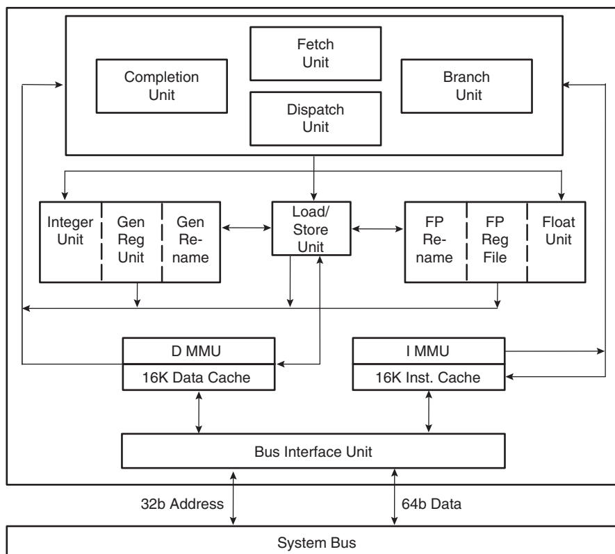
Figure 3-1. Block Diagram
