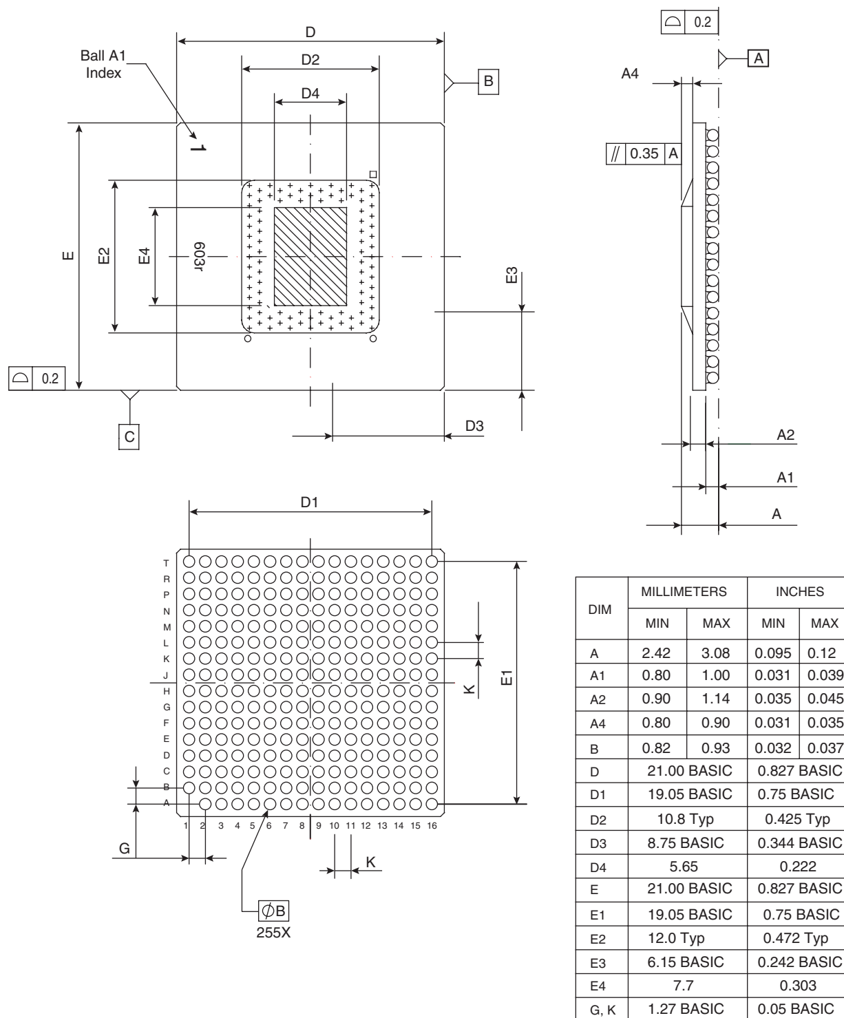
Figure 15-1. Mechanical Dimensions of the HiTCE CBGA Package
