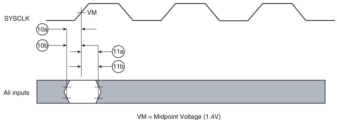
Figure 11-2. Input Timing Diagram
