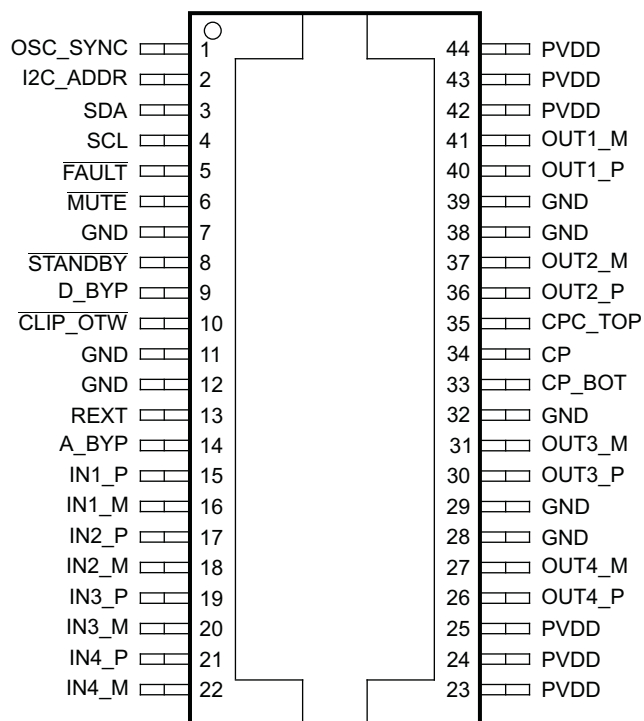
TAS5424A DKD Package (Top View)
